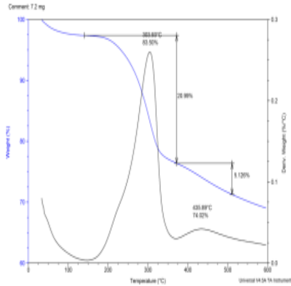
Figure 1. Sample 1 paper, with wollastonite and with starch
