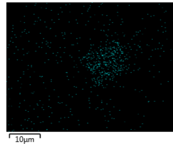
K K \alpha 1
